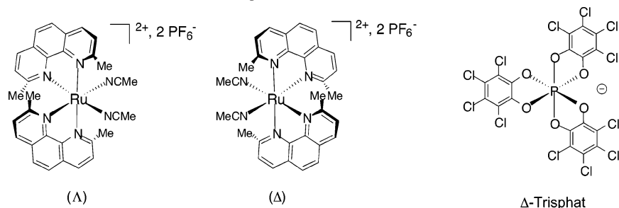
Chart 1. Structures of the Two Enantiomers of Ruthenium Complex 1 [PF 6 ] 2 and of the Trisphat Anion of Δ Configuration
