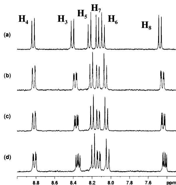
Figure 3. Aromatic region of the ^1\text{H} NMR spectrum of the racemic cis - [\text{Ru}(\text{dmp})_2(\text{CH}_3\text{CN})_2][\text{PF}_6]_2 complex, 1 [\text{PF}_6]_2 , (a) in the absence and in the presence of (b) 1, (c) 2, and (d) 4 equiv of [\textit{n}\text{-Bu}_3\text{NH}][\Lambda\text{-Trisphat}] , in acetone- d_6 .
