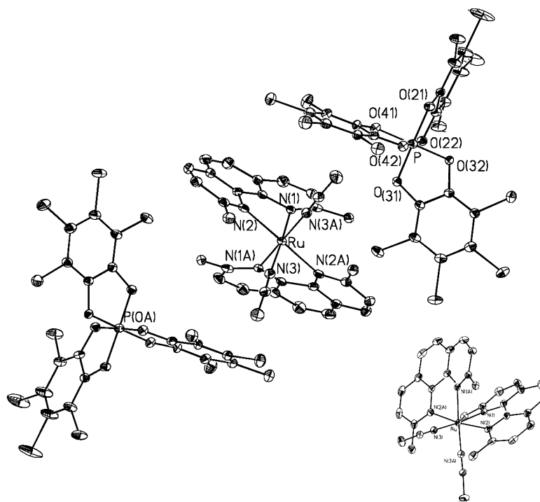
Figure 5. X-ray structure of cis -[ \Lambda -Ru(dmp) _2 (CH _3 CN) _2 ][ \Delta -Trisphat] _2 ·10H _2 O·2CH _2 Cl _2 . Hydrogen atoms have been omitted for clarity. Inset: ORTEP representation of the [ \Lambda -Ru(dmp) _2 (CH _3 CN) _2 ] ^{2+} cation.
